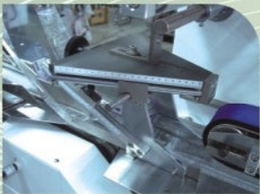
Adjustable Bag Former
